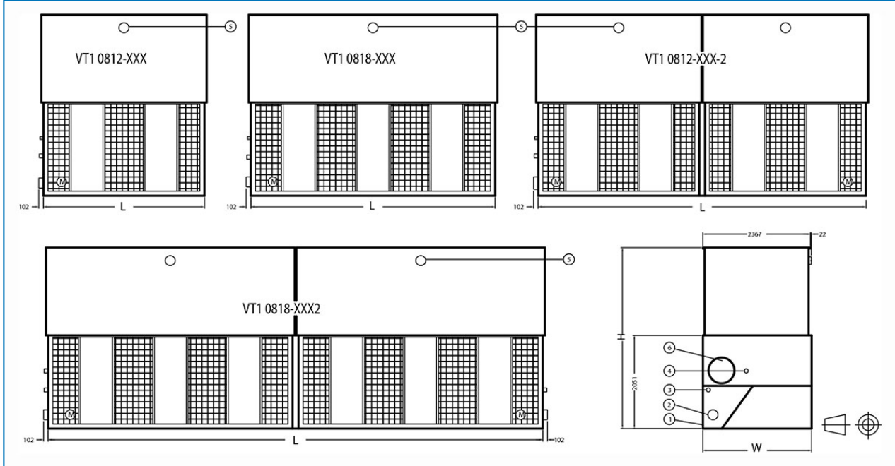
1. Drain ND 50; 2. Water Outlet; 3. Overflow ND50; 4. Make Up ND25; 5. Water Inlet; 6. Access Door.
