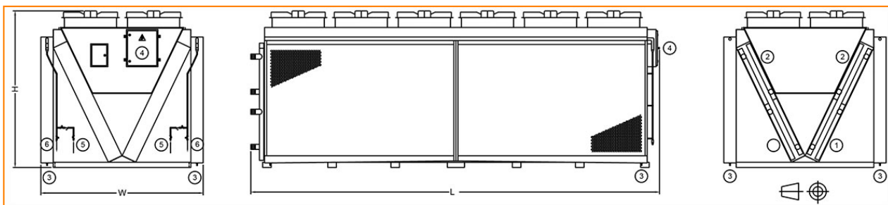
1. Fluid inlet connection; 2. Fluid outlet connection; 3. Pre-cooler water drain; 4. Electrical panel; 5. Pre-cooler city water connection; 6. Pre-cooler pad.
