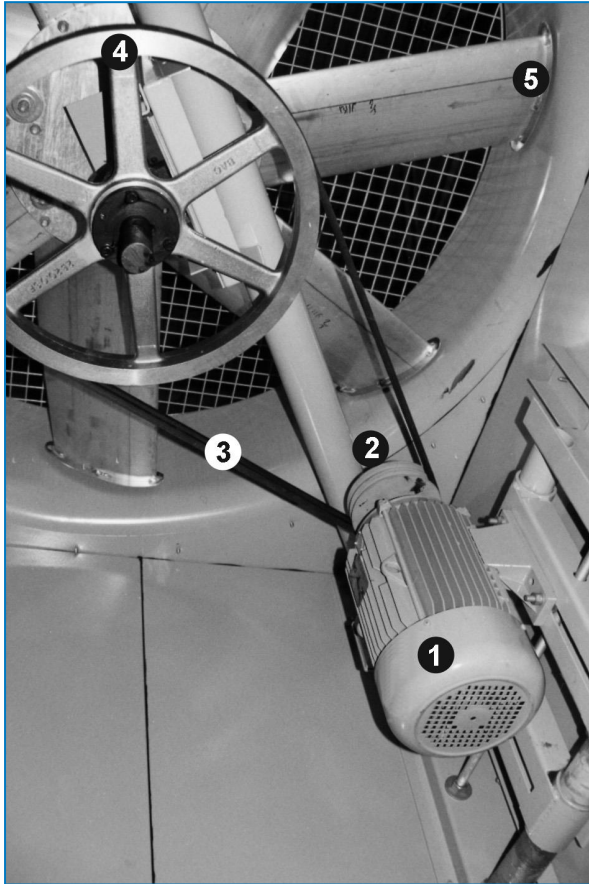
Drivsystem
