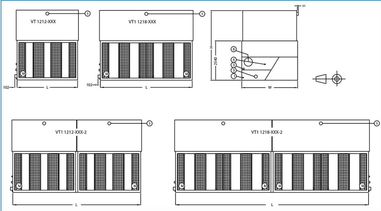
1. Drain ND 50; 2. Water Outlet; 3. Overflow ND50; 4. Make Up ND25; 5. Water Inlet; 6. Access Door.
