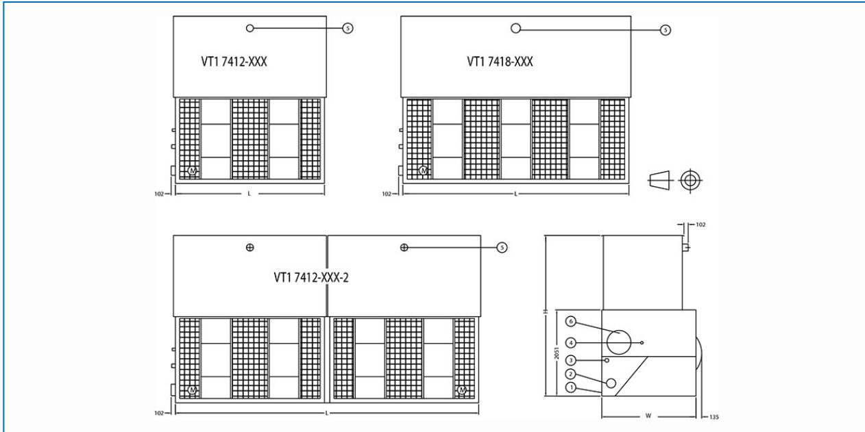
1. Drain ND 50; 2. Water Outlet; 3. Overflow ND50; 4. Make Up ND25; 5. Water Inlet; 6. Access Door.
